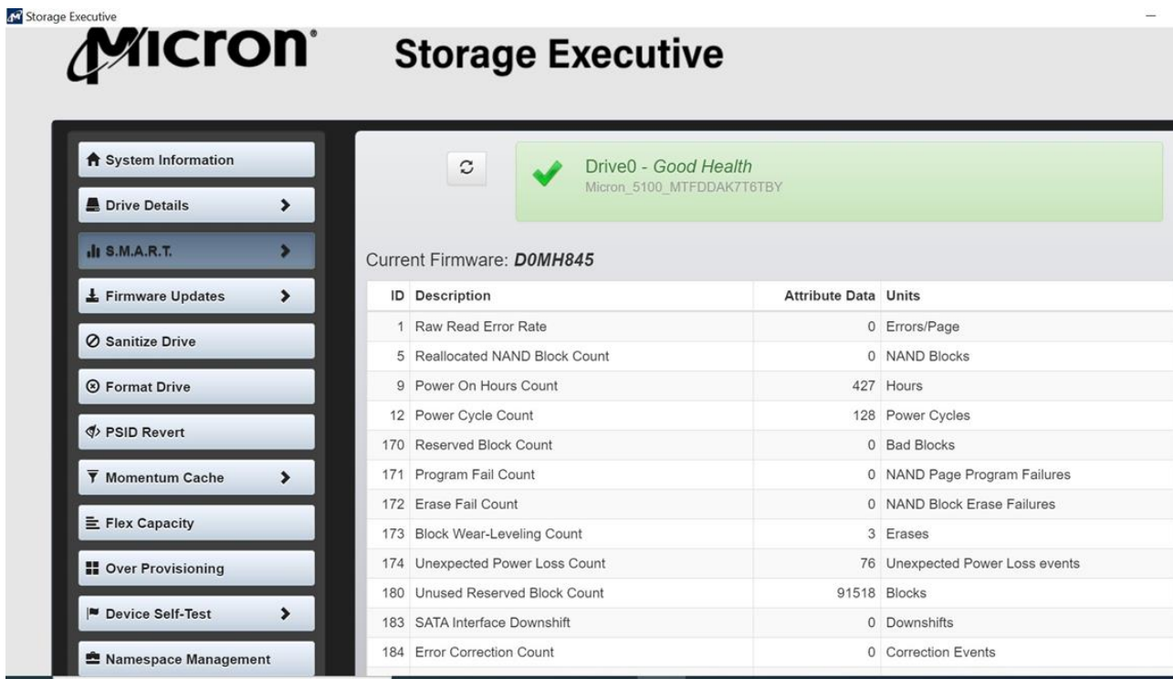
Fig: 11 SMART Attributes
